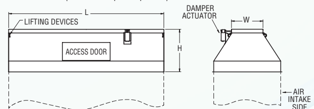
Tapered Discharge Hood (See page 21 for dimensions)
