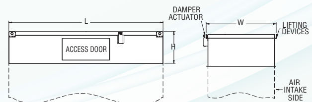
Straight-Sided Discharge Hood (See page 21 for dimensions)
